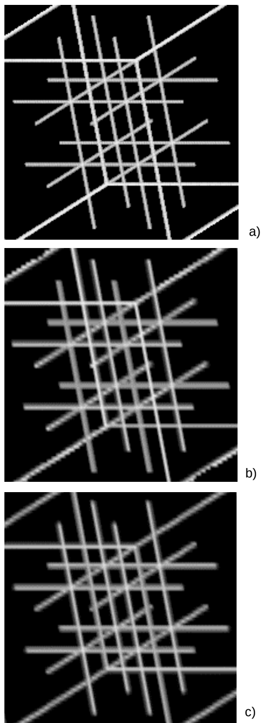
Figure 11. Rendering a phantom in "high" quality with a) ray-casting b) projective shear-warp c) splatting shear-warp
