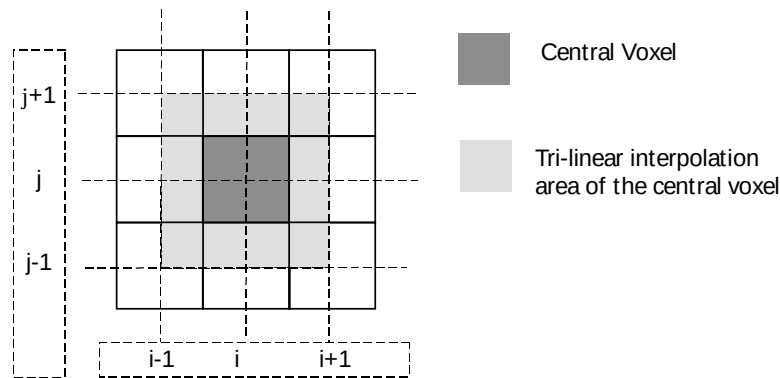
Figure 4. The areas influenced by the central voxel ( i, j ) during a tri-linear Interpolation
